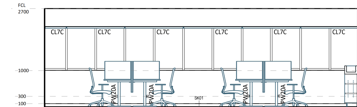
2 ELEVATION DETAIL 1 : 50
