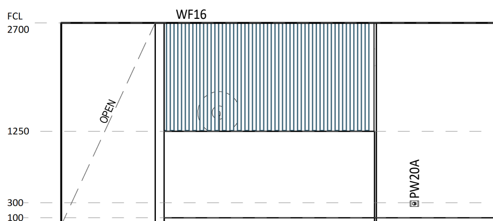
10 ELEVATION DETAIL 1 : 50
