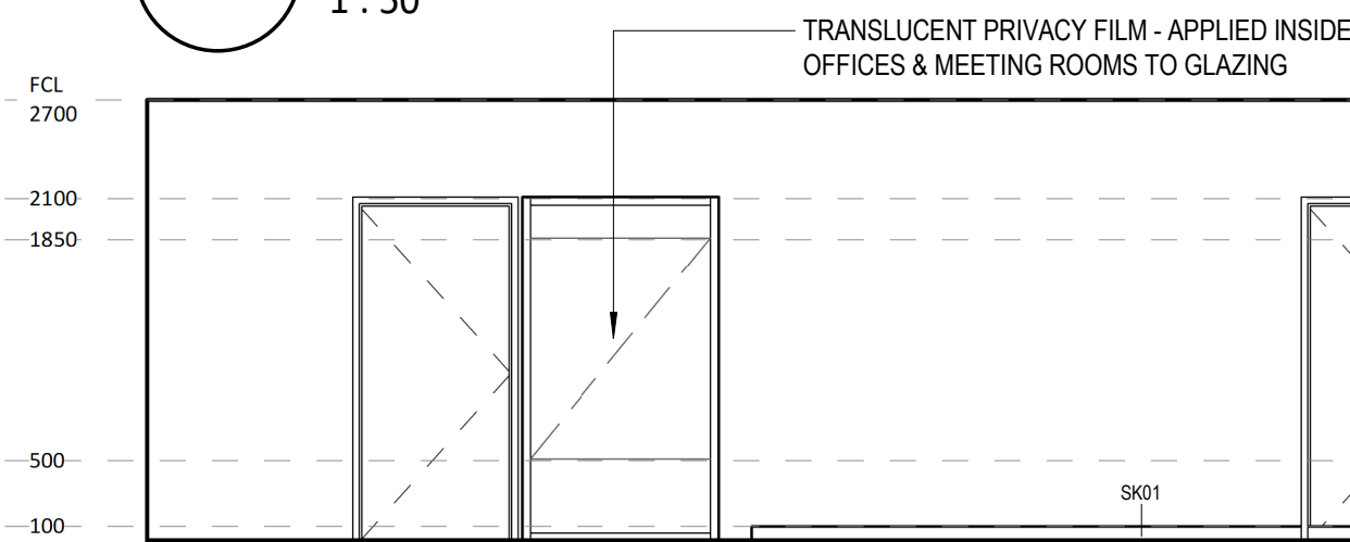
4 ELEVATION DETAIL 1 : 50
