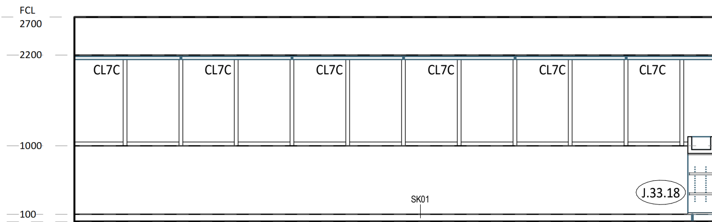
7 ELEVATION DETAIL 1 : 50
